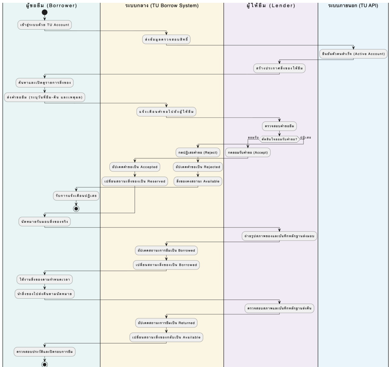
Activity Diagram
